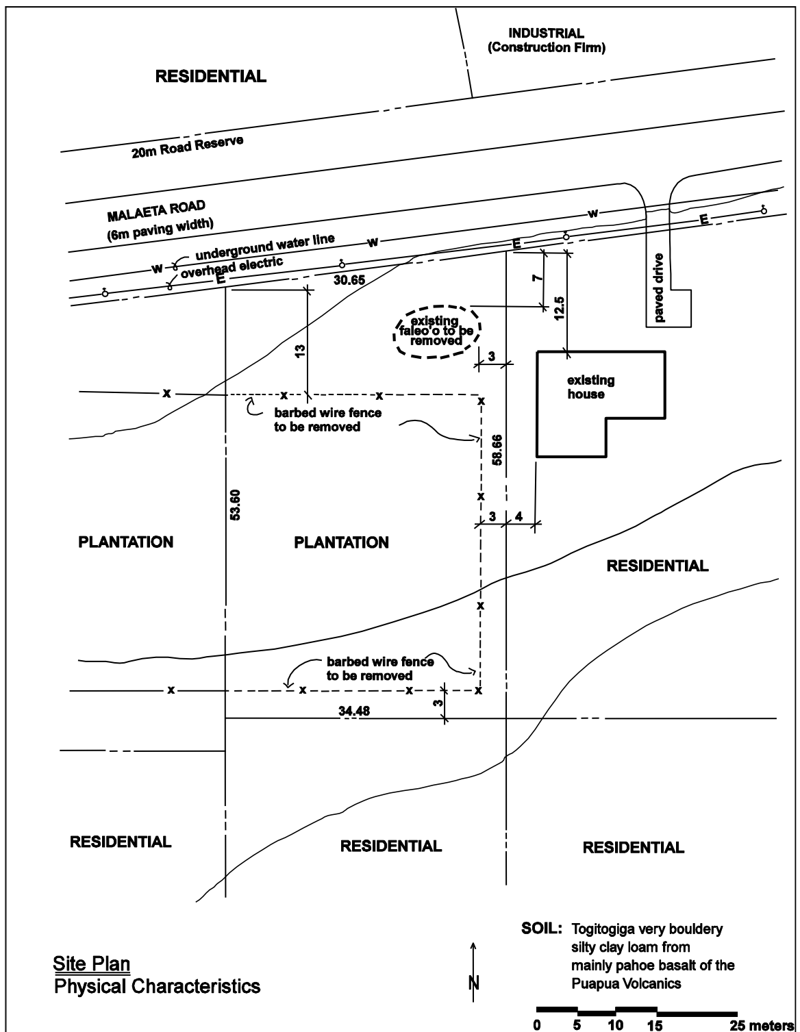
Figure 3: Site Plan Illustrating Physical Characteristics
