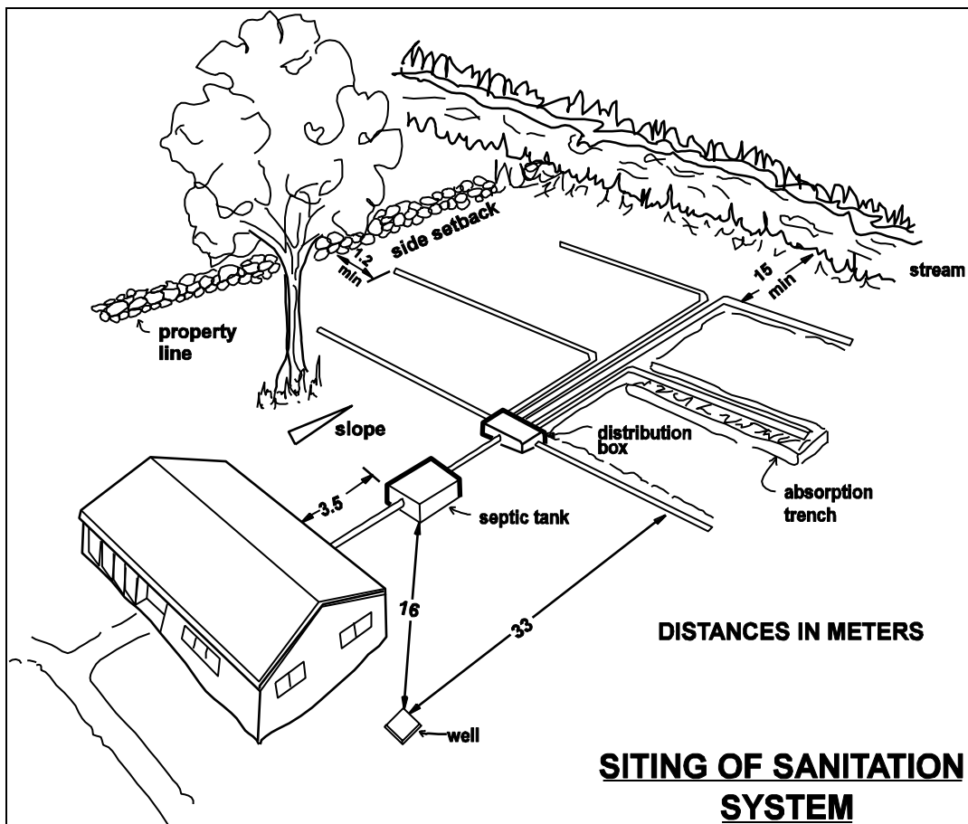
Figure 8: Siting of Sanitation System
